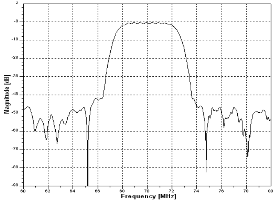
Frequency Response
